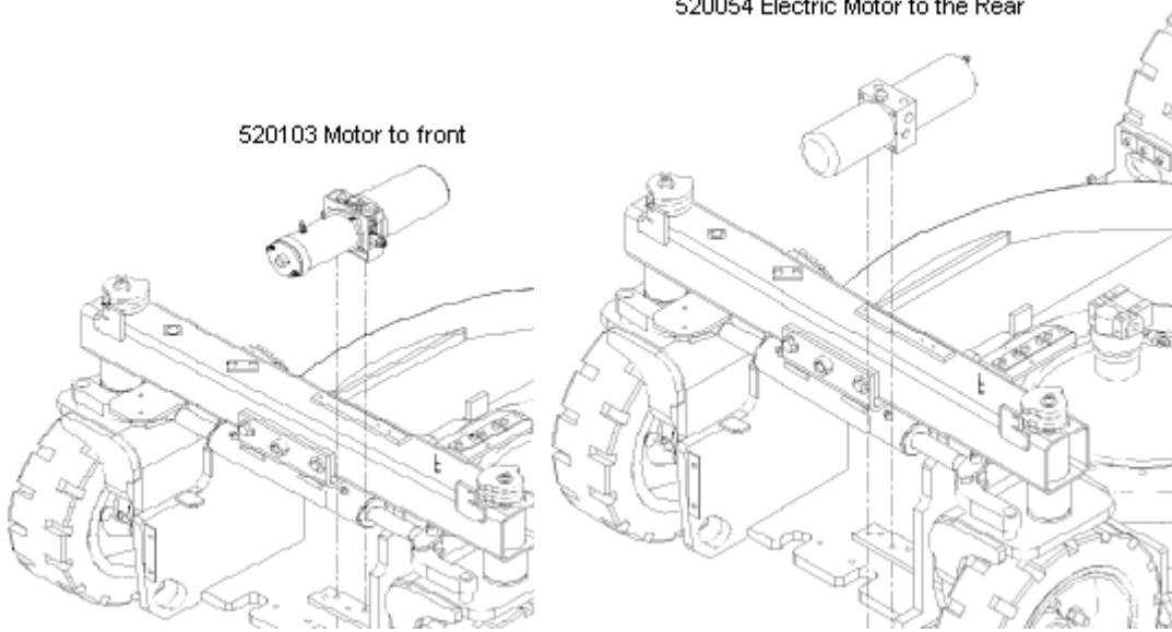
520054 Electric Motor to the Rear
